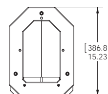
TOP VIEW [POLE MOUNT is on BOTTOM]
